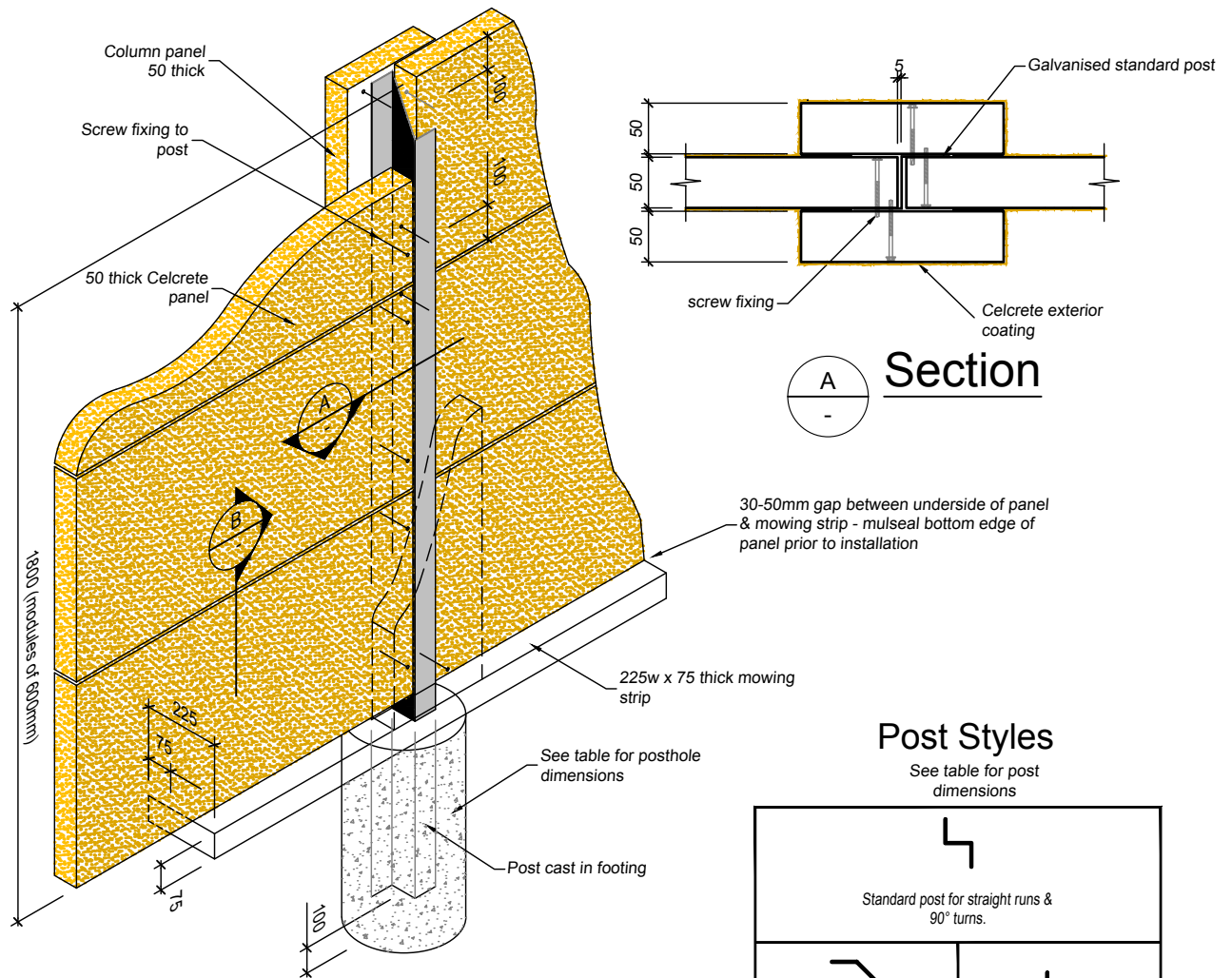
ISOMETRIC VIEW OF CELCRETE FENCE
